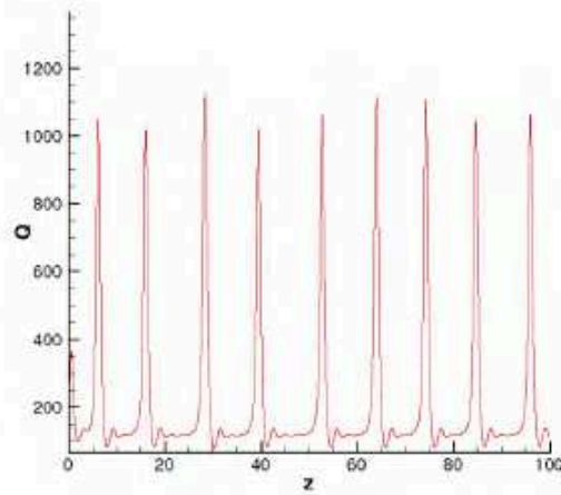
Figure 10. Exploding soliton: evolution of the energy which shows periodic bursts and recovery.
