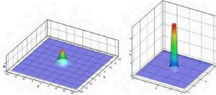
Figure 1. Initial condition. Left: Gaussian shape. Right: ring vortex with vorticity m = 1 .
