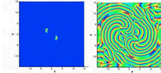
Figure 6. Spinning “bean-shape” soliton with elliptic vortex initial condition m = 1 , \epsilon = -0.17 , z = 50 . Left: contour plot of amplitude. Right: phase plot.
