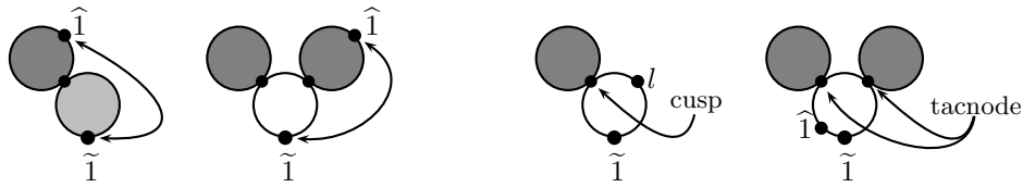
Figure 7: Some boundary strata of \overline{\mathcal{V}}_1^{(1)}(\mu)
