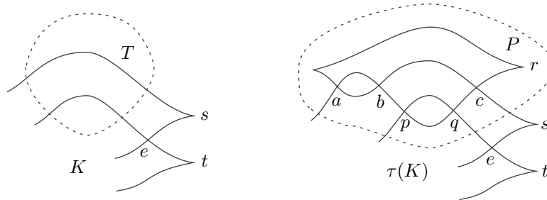
(a) Special Legendrian knot
