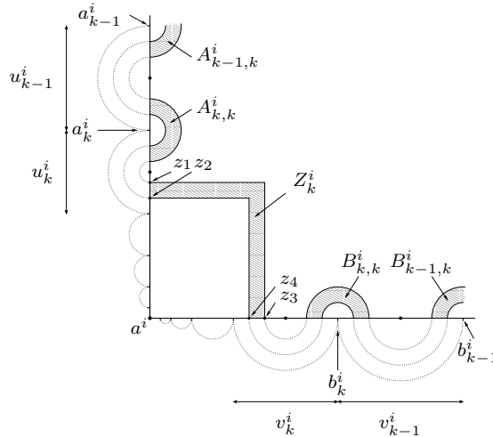
Figure 32: The rectangular quarter-annulus Z_k^i
