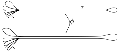
Figure 5: The invariant train track for the horseshoe
