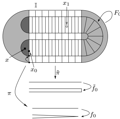
Figure 3: The horseshoe map
