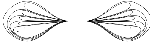
Figure 9: W^+ and W^-
