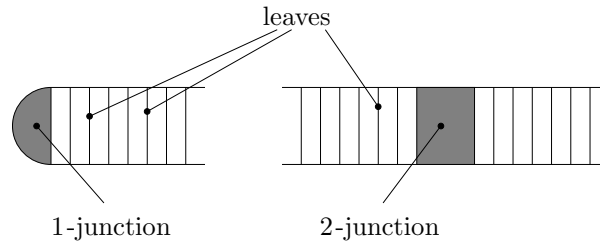
Figure 2: Charts in a thick interval
