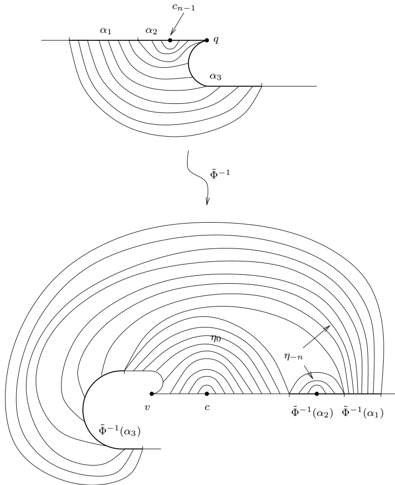
Figure 29: The arc bands in case c)
