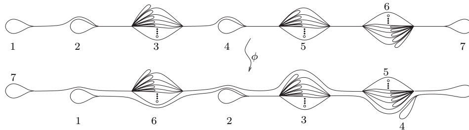
Figure 20: The generalized train track corresponding to s = 1000(101)^\infty and its image
