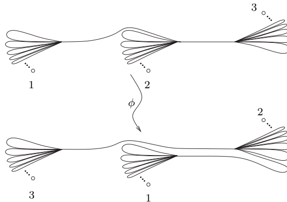
Figure 12: The generalized train track corresponding to s = \text{lhe}(1/3) and its image
