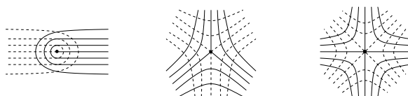
Figure 1: Pronged singularities of the invariant foliations
