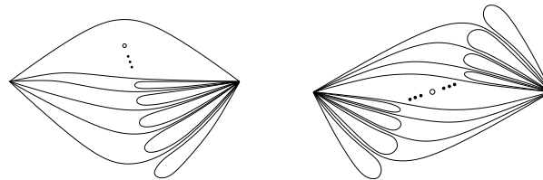
Figure 18: Extra bubbles: the configurations V_1^+ B and V_2^- B^2
