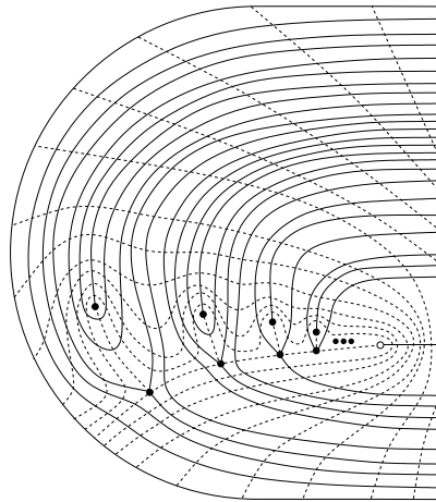
Figure 25: Detailed view of the shaded regions of Figure 24
