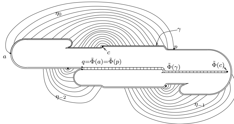
Figure 26: \mathcal{R} and its image under \tilde{\Phi}
