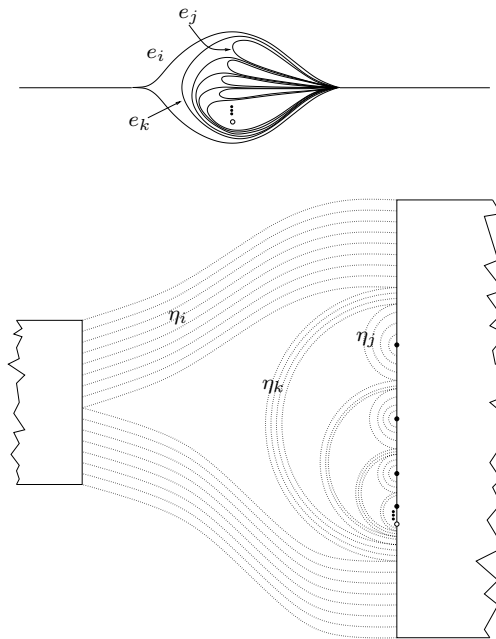
Figure 23: The arc bands in the junction between R_3 and R_4
