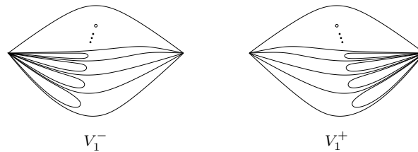
Figure 16: V_1^- and V_1^+
