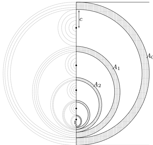
Figure 34: Annuli with divergent moduli sum surrounding an accumulation of singularities of type W .
