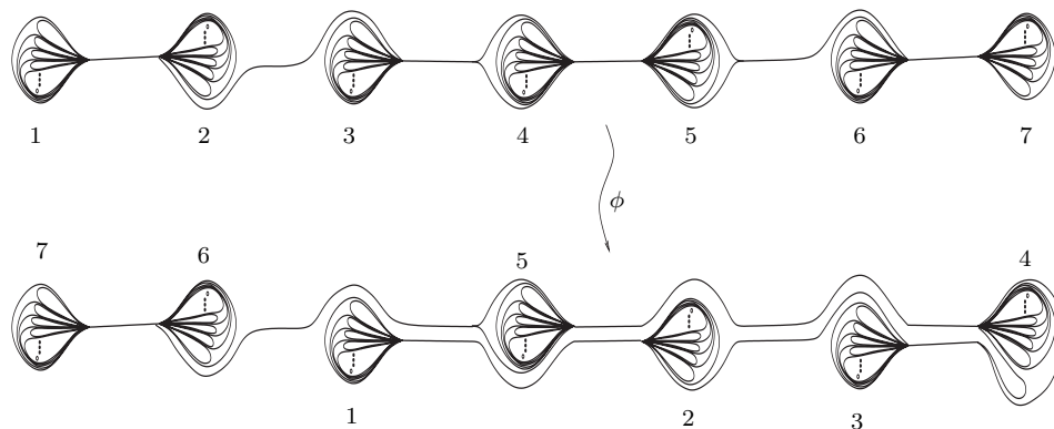
Figure 14: The generalized train track corresponding to s = (1001011)^\infty and its image
