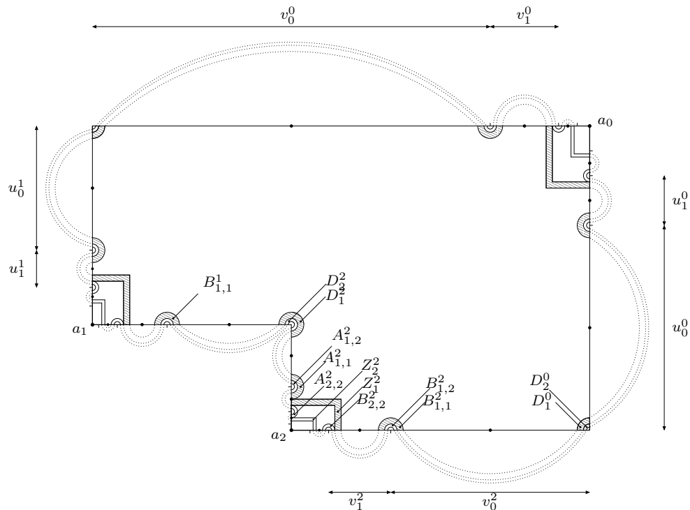
Figure 33: Annuli with divergent moduli sum surrounding the accumulation of singularities of \Phi_{\text{lhe}(1/3)}
