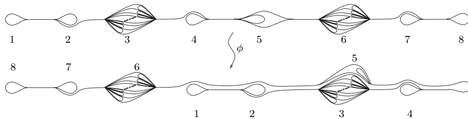
Figure 21: The generalized train track corresponding to s = 100101(10)^\infty and its image
