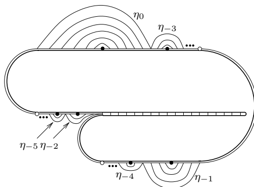
Figure 27: The arc bands in case a): here s = (101)^\infty = \text{lhe}(1/3)
