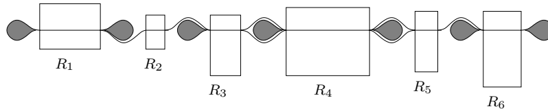
Figure 22: The rectangles R_i placed along the real edges of \tau
