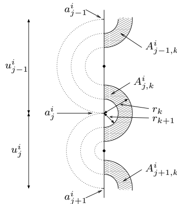
Figure 31: The half-annuli A_{j,k}^i
