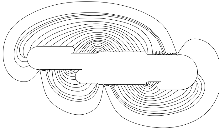
Figure 30: The complete second stage decomposition for the running example
