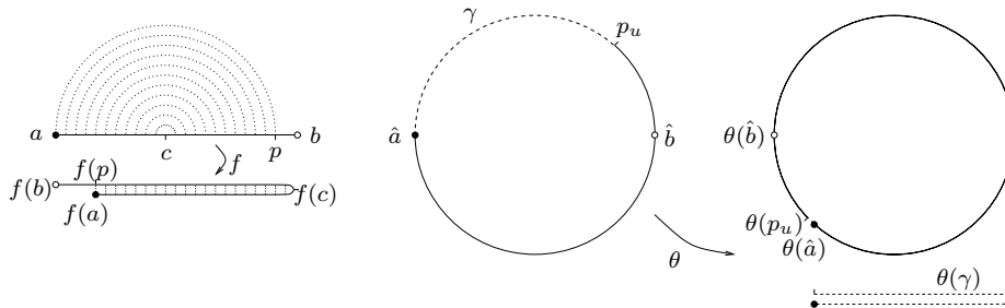
Figure 8: A unimodal map and the induced outside map
