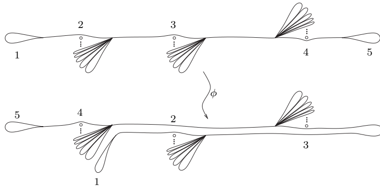
Figure 19: The generalized train track corresponding to s = \text{rhe}(1/3) and its image
