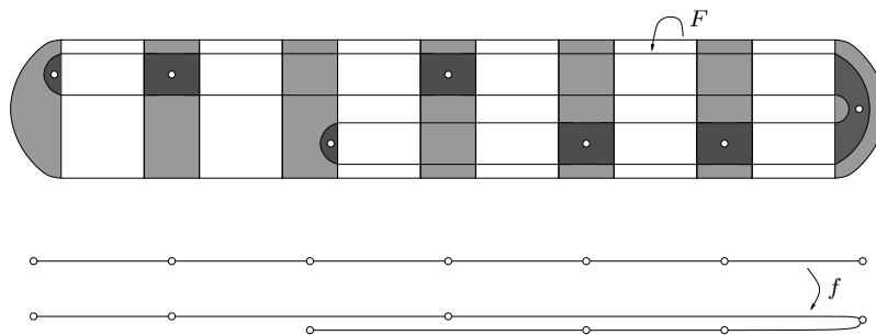
Figure 4: A thick interval map associated to a horseshoe periodic orbit
