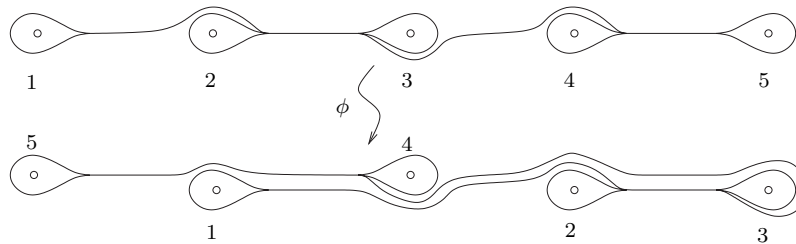
Figure 13: The generalized train track corresponding to s = \text{NBT}(1/3) and its image
