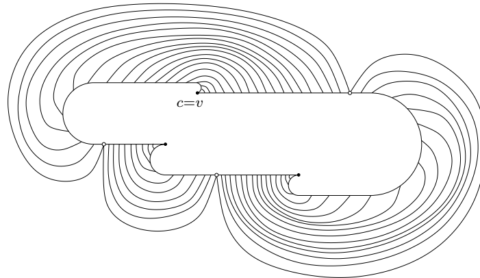
Figure 28: The arc bands in the NBT case: here s = (10011)^\infty
