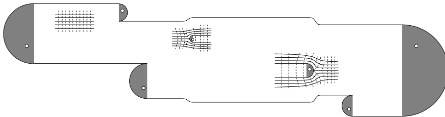
Figure 24: The quotient disk \mathcal{R} and its foliation
