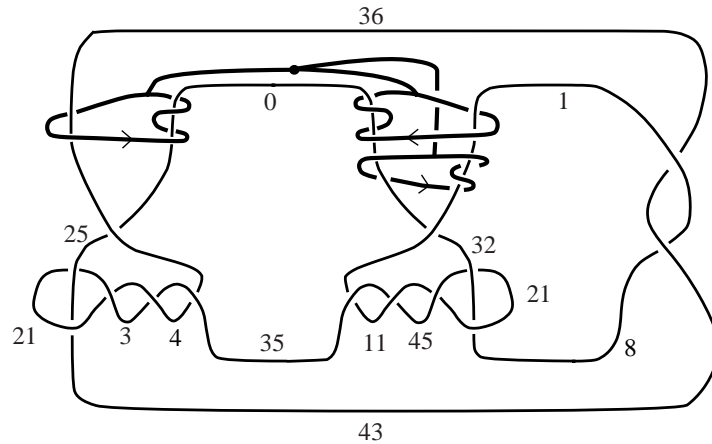
Figure 5: The representation \bar{\chi}: \pi_1(S^3 - K) \rightarrow G
