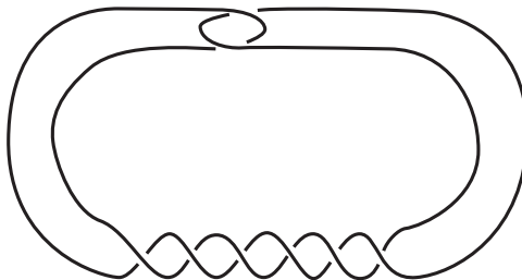
Figure 2: A twisted double of the unknot
