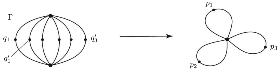
Figure 4: The double cover \Gamma \rightarrow S^1 \vee S^1 \vee S^1 , corresponding to the homomorphism \text{Free}_3 \rightarrow \mathbb{Z}/2\mathbb{Z} , sending each “preferred” generator to the non-trivial element.
