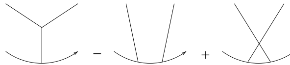
Figure 6: STU relation
