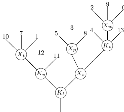
Figure 6: Typical coloured n -planar tree. Here v, w, p, t, s are n -ordinals decorating vertices.
