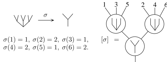
Figure 4: A 2-ordinal and its corresponding 2-planar tree.
