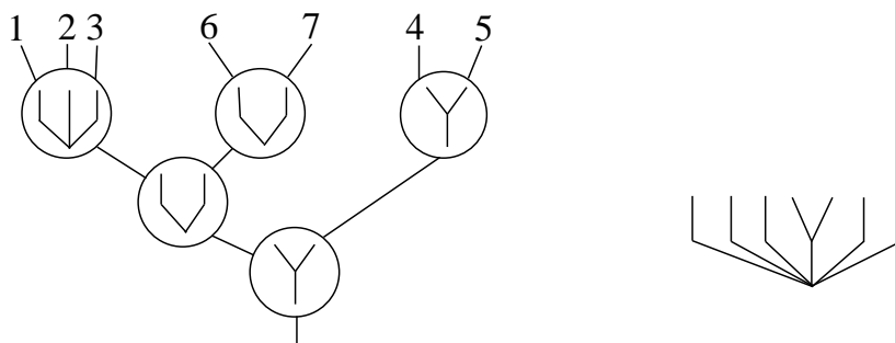
Figure 8: A 2-planar tree as a labelled decorated tree with dominating 2-ordinal.
