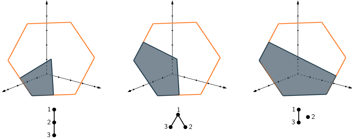
Figure 1: Pictured are each of the two dimensional poset permutahedra other than the permutahedron itself up to symmetry with their corresponding posets.
