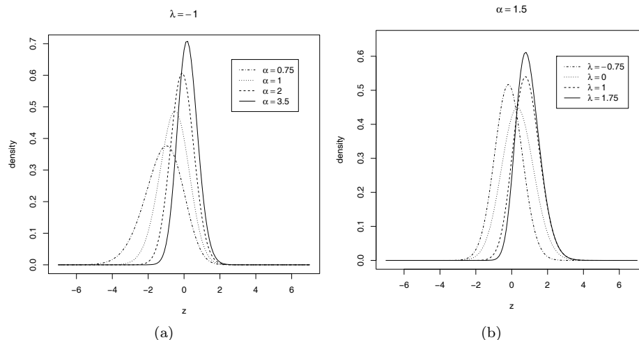
FIGURE 1: Probability density function of the skew-normal alpha-power distribution.
