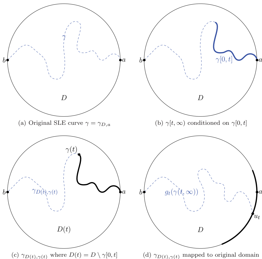
Fig 2: Domain Markov property
