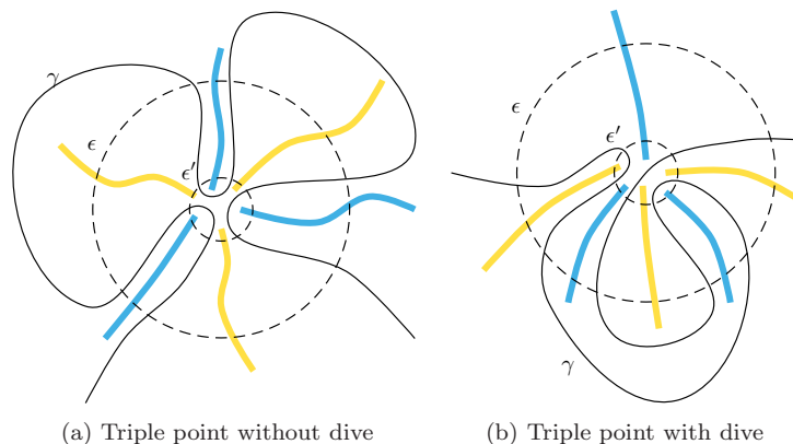
Fig 10: Interior triple point and six-arm event
