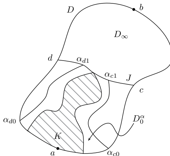
Fig 9: Crosscut and hull distribution
