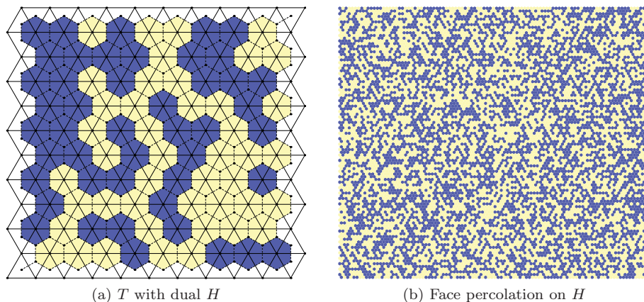
Fig 5: Site percolation on T as face percolation on H
