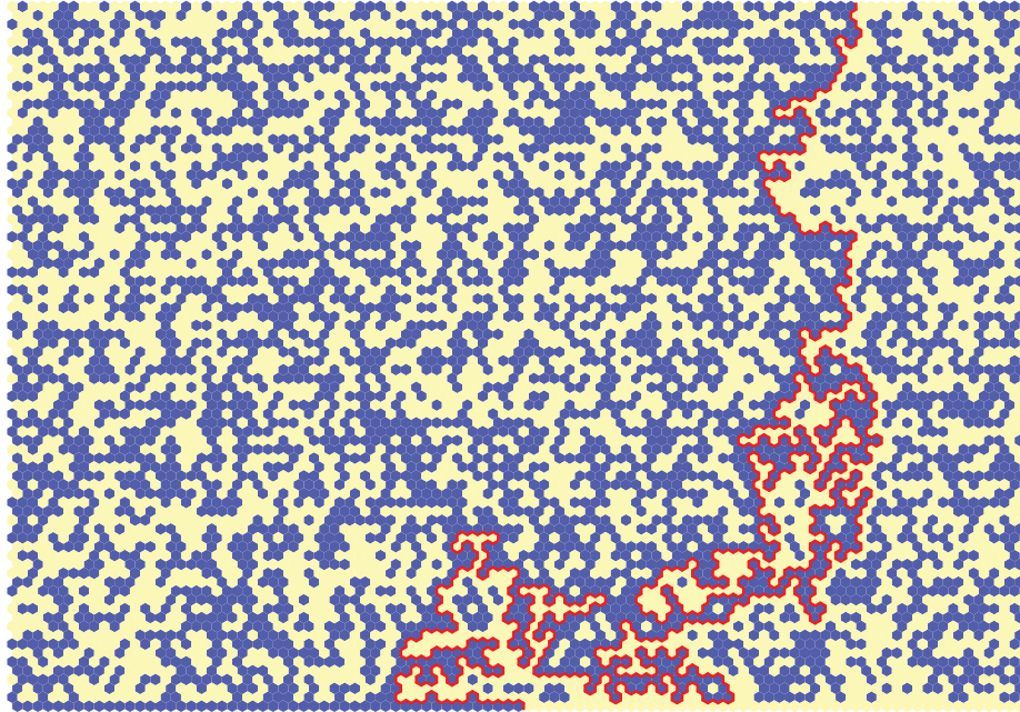
Fig 3: Percolation exploration path
