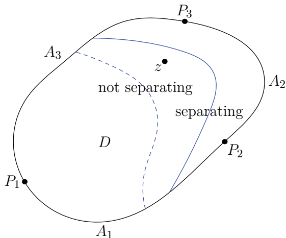
Fig 6: Schematic of separating event E_2(z)
