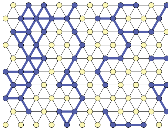
Fig 1: Site percolation on T
