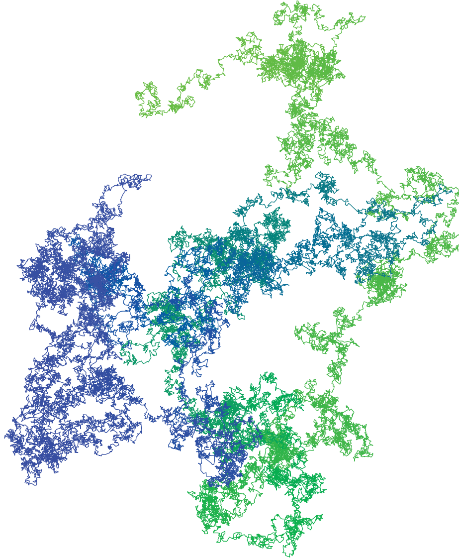
Fig 4: Approximate sample path of Brownian motion
