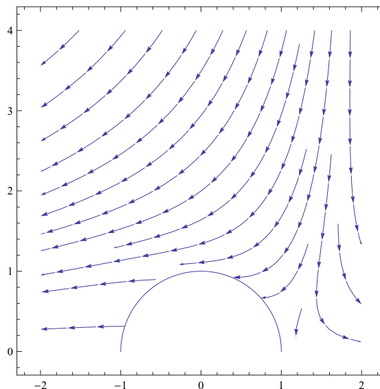
Fig 8: Vector field 2/[g_{\mathbb{D}}(z) - 2] around \mathbb{D}
