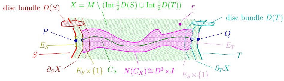
FIGURE 12. Illustration for the proof of Proposition 11.1.
