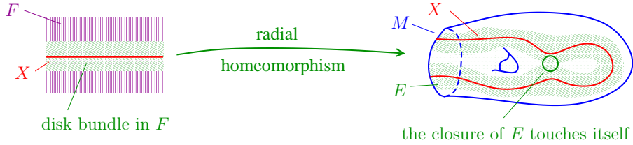
FIGURE 6. Non-extendable internal linear bundle.
