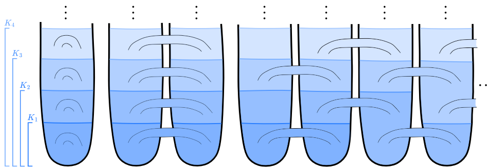
FIGURE 3. A 1-sliced, a 2-sliced, and an \infty -sliced Loch Ness monster with the noncompact boundary components represented by the bold lines. The blue shading represents a given compact exhaustion \{K_i\} for each surface.
