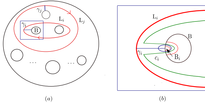
FIGURE 2. (a) A planar open book and the disjoint arcs. (b) Enlarged view of the region inside the box in disjoint arcs lying "to the right".
