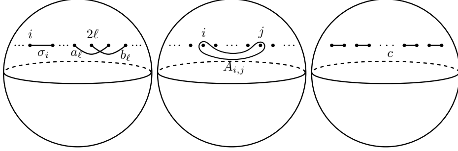
FIGURE 3. Left to right: the arcs about which \sigma_i , a_\ell , and b_\ell are half-twists, the curve about which A_{i,j} is a Dehn twist, and the collection of arcs about which c is a composition of half-twists. The labels above the marked points are to indicate the enumeration.
