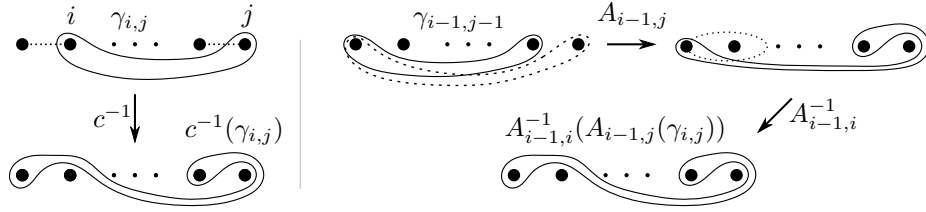
FIGURE 4. Both i and j are even. The left figure shows \gamma_{i,j} and its image under c^{-1} , which is a product of half-twists about the dashed arcs. Starting at the top left and going clockwise, the right figure shows \gamma_{i-1,j-1} , A_{i-1,j}(\gamma_{i-1,j-1}) , and A_{i-1,i}^{-1}(A_{i-1,j}(\gamma_{i-1,j-1})) . The dashed curves indicate the curves about which A_{i-1,j} and A_{i-1,i}^{-1} are Dehn twists.
