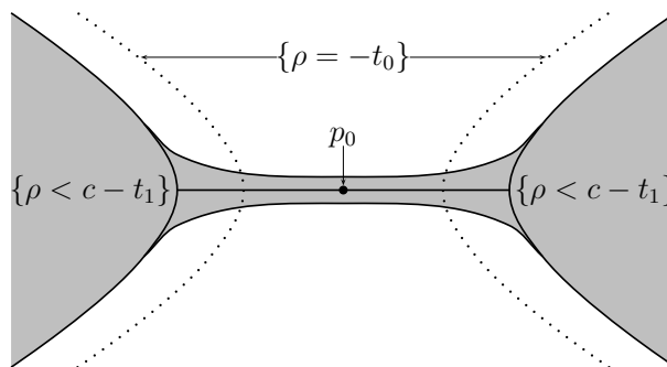
FIGURE 1. Passing a critical level of \rho .
