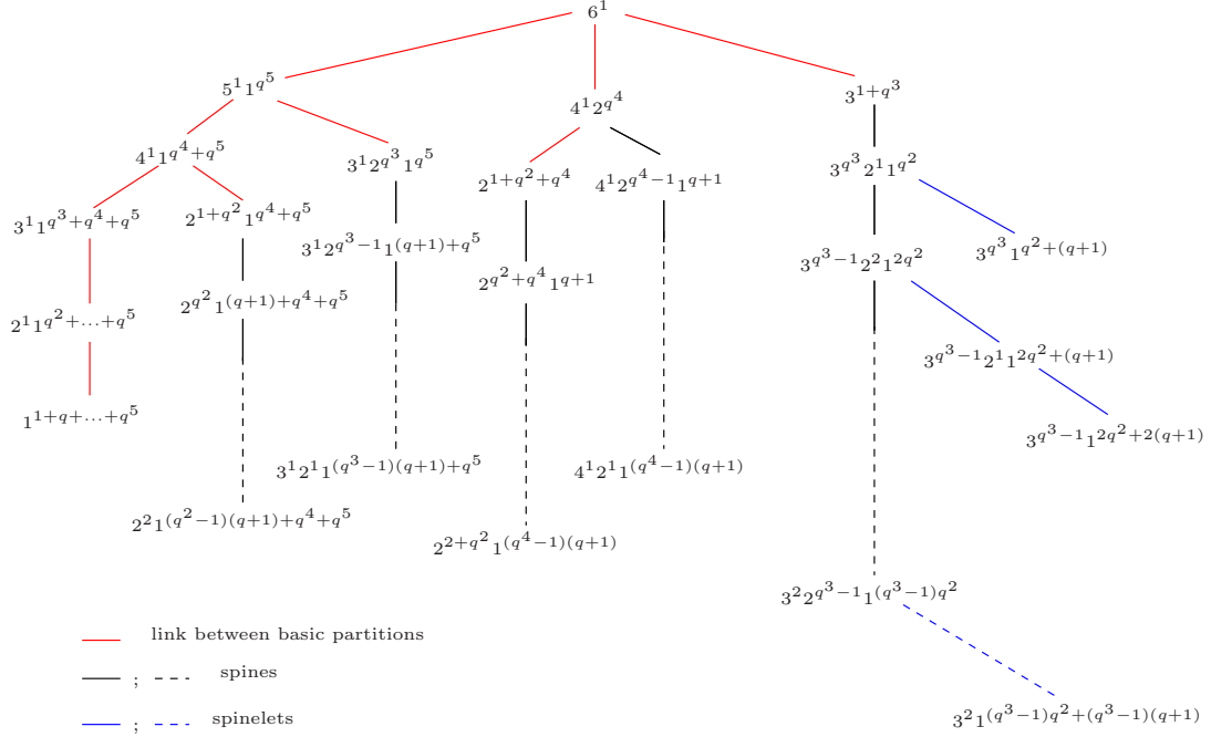
Figure 1: Basic Gaussian partitions, spines, and spinelets for n = 6
