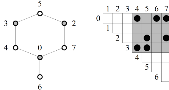
Figure 2: Triangular representation of an \alpha -labeling
