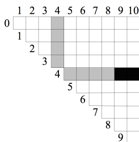
Figure 4: Counting of deleted cells
