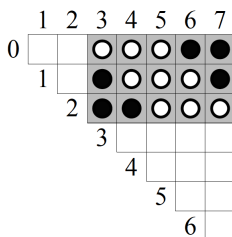
Figure 3: Triangular arrangements for n = 7 and \lambda = 2
