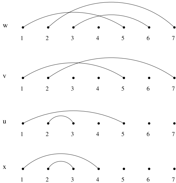
Fig. 1 Illustration for the proof of Proposition 3.9
