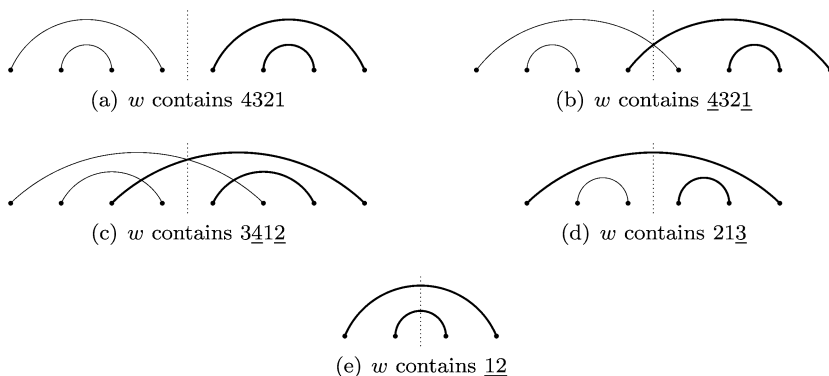
Fig. 3 Graph representations for 4321-containing \phi(w)
