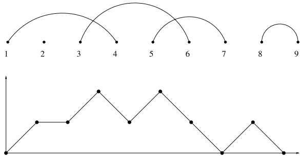
Fig. 5 A Boolean involution and the corresponding restricted Motzkin path
