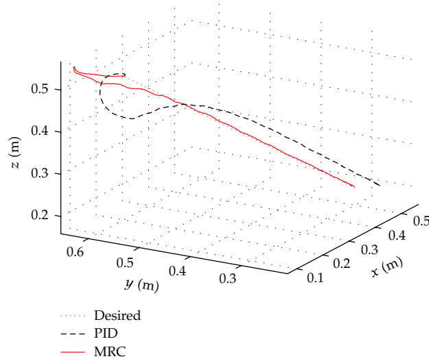
Figure 8: Task space ( xyz ) trajectories for the straight line trajectory in an uncertain and disturbed condition.
