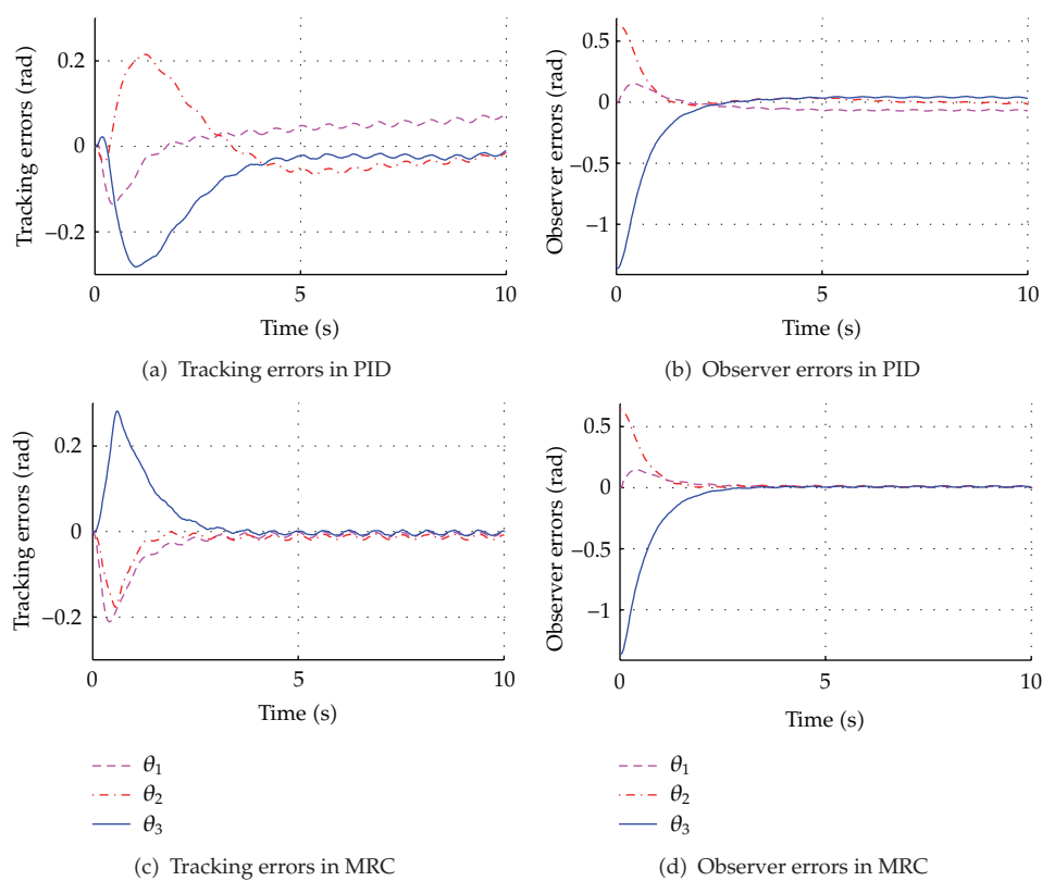
Figure 6: Time trajectories of the joint position errors for the straight line trajectory in an uncertain and disturbed condition.
