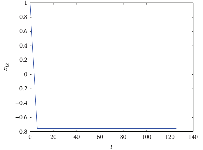
FIGURE 5: Numerical results for (77) with c_1 = 0 . k = 20 .
