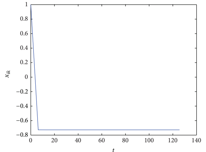
FIGURE 7: Numerical results for (77) with c_1 = 1 . k = 20 .
