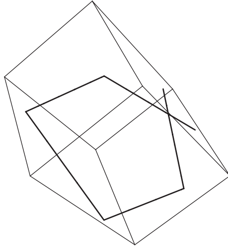
Figure 3: The Kahan's integrator of the system (3.8) ( c_1 = 1, c_2 = 2, c_3 = 3, k = 10 , and h = 1, x_1(0) = x_2(0) = x_3(0) = 1 ).
