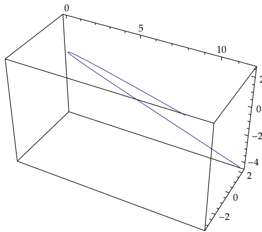
Figure 4: The Lie-Trotter integrator of the system (3.8) ( c_1 = 1, c_2 = 2, c_3 = 3, k = 10 , and x_1(0) = x_2(0) = x_3(0) = 1 ).
