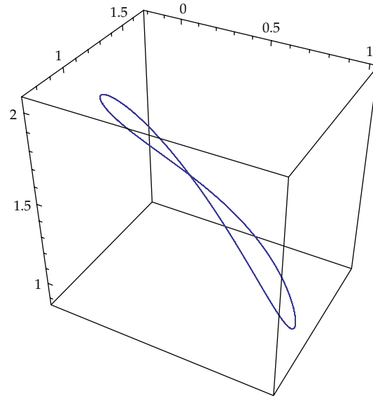
Figure 2: The 4th-step Runge-Kutta integrator of the system (3.8) ( c_1 = 1, c_2 = 2, c_3 = 3, k = 10 , and x_1(0) = x_2(0) = x_3(0) = 1 ).
