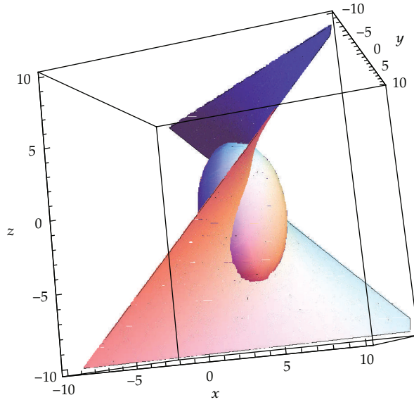
Figure 1: The phase curves of the system (3.8) ( c_1 = 1, c_2 = 2, c_3 = 3, and k = 10 ).
