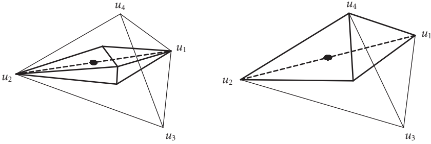
Figure 3.4. Two horoballs centered at (u_1 + u_2)/2 with \pi(g_{\{3,4\}}) equal to (u_3 + u_4)/2 on the left and u_4 to the right.
