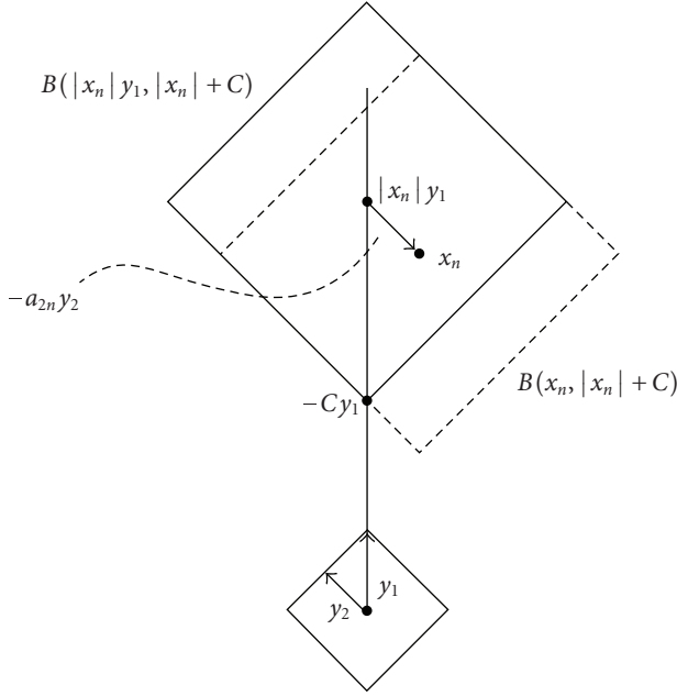
Figure 4.1. The decomposition of x_n .
