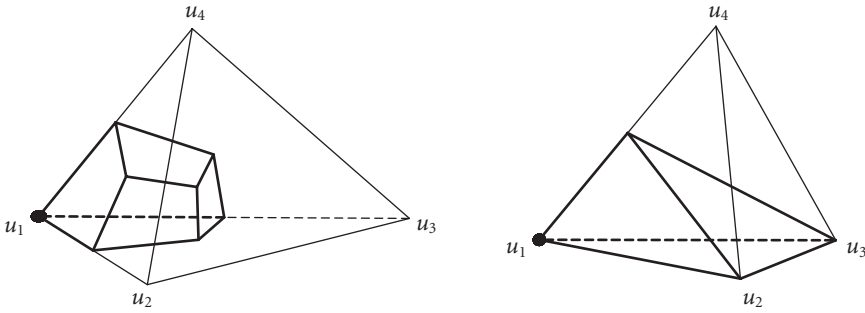
Figure 3.3. Two horoballs centered at u_1 with \pi(g_{\{2,3,4\}}) equal to (u_2 + u_3 + u_4)/3 on the left and (u_2 + u_3)/2 on the right.
