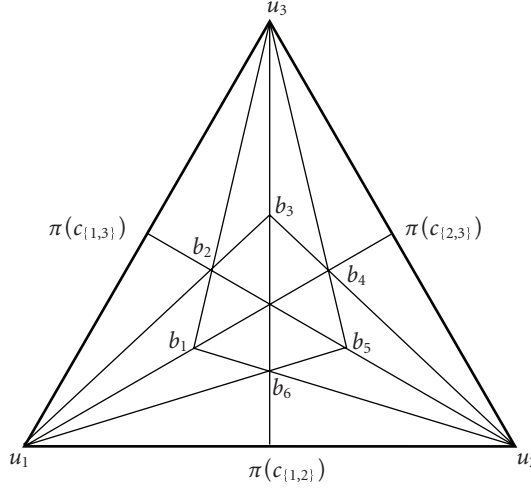
Figure 3.1. The k -ball in \Delta centered at c with extremal points b_1, \dots, b_6 .
