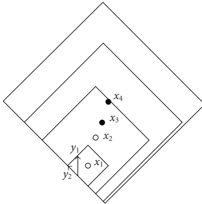
Figure 3.5. Blowing up and shifting a sequence of balls.
