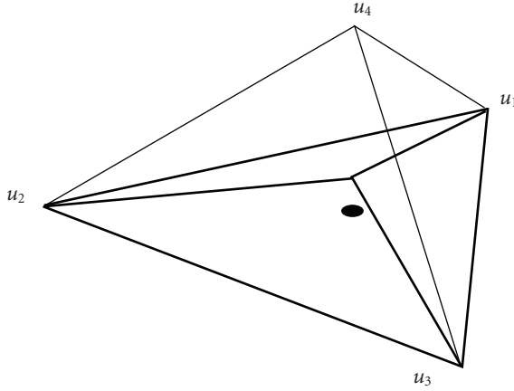
Figure 3.2. A horoball centered at (u_1 + u_2 + u_3)/3 .
