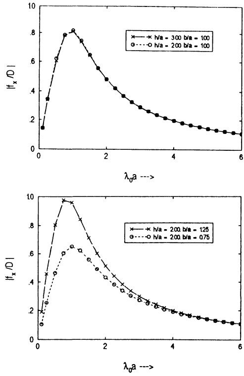
FIGURE 3. Non-dimensional horizontal force.
