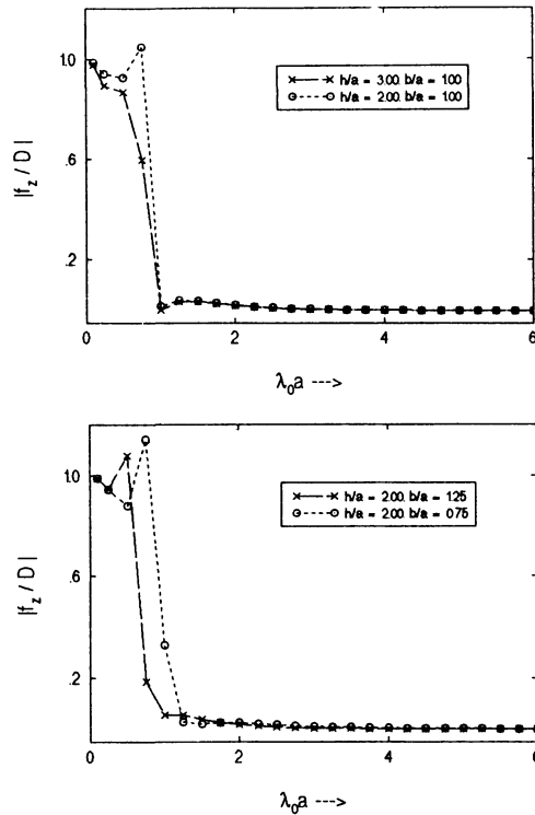
FIGURE 4. Non-dimensional vertical force.
