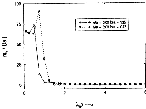
FIGURE 6. Non-dimensional moment, \frac{m_b}{Da} .
