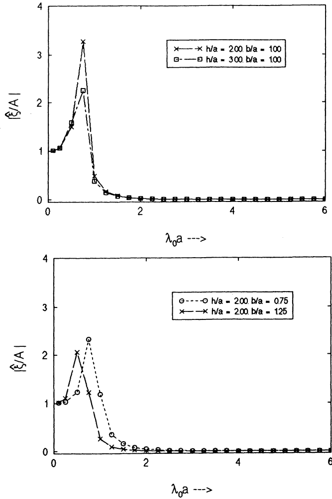
FIGURE 2. Amplitude of \hat{\xi}/A .
