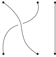
Figure 1.1. braid \sigma .
