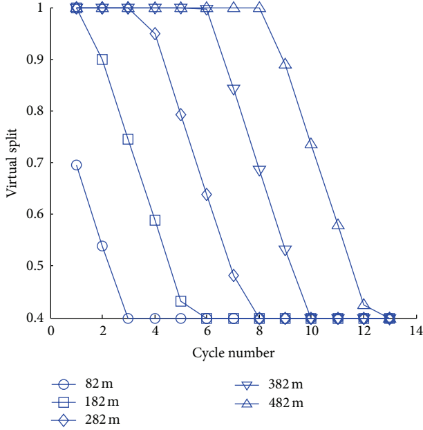
FIGURE 12: Virtual split propagation, C = 100 s, g = 40 s, r = 50 s, q = 1000 ve/h, k_j = 180 veh/km, q_m = 1800 veh/h.
