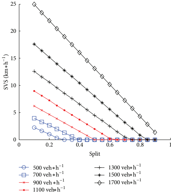
FIGURE 16: SVS versus split with triangular fundamental diagram; k_j = 180 veh/km, q_m = 1800 veh/h, v_f = 50 km/h, and w_a = 12.5 km/h.
