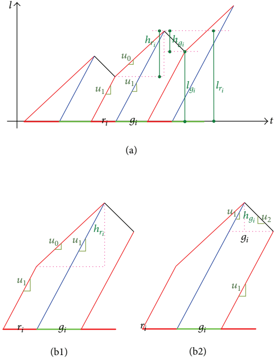
FIGURE 7: Stopping wave and starting wave with insufficient split.
