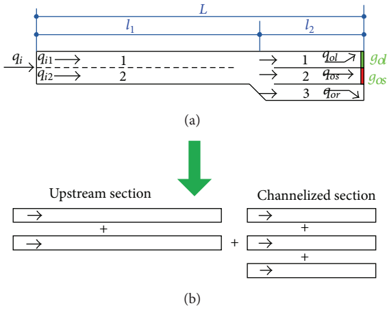
FIGURE 6: Sketch map of basic road and its decomposition.
