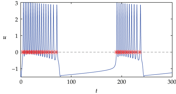
FIGURE 2: Time series of the u state of an active \beta cell as the master system with (1) for some iterations in time. The gray dashed line marks the Poincaré plane, and each crossing event is marked with red asterisks.
