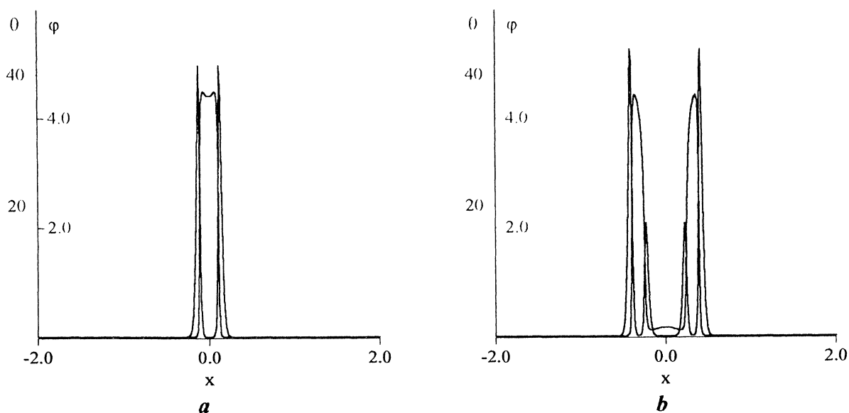
FIGURE 1 Stages of streation development in one-dimensional plane case at the \theta_0 = 3.0 nM, \varphi_0 = 0.065 nM. The other parameters were fixed at the following values \alpha = 2.0 min ^{-1} , \beta = 0.0015 min ^{-1} , \gamma = 5.00 min ^{-1} nM ^{-1} , C = 5.0 nM, \kappa_1 = 0.05 min ^{-1} , \kappa_2 = 0.35 min ^{-1} , D_1 = D_2 = 0.0006 mm ^2 min ^{-1} . The red curve is the inhibitor distribution, the blue one is that of activator. Domain size L = 2 mm, number of grid points N = 300 , step of time integration was 0.01 min.
