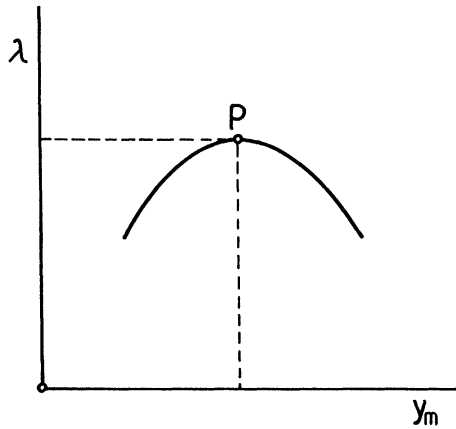
FIGURE 6 A bifurcation diagram with turning point P .
