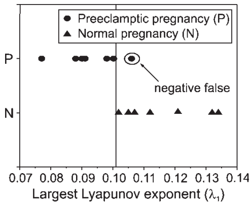
FIGURE 3 Estimated values of the largest Lyapunov exponent obtained from the original HR recordings.
