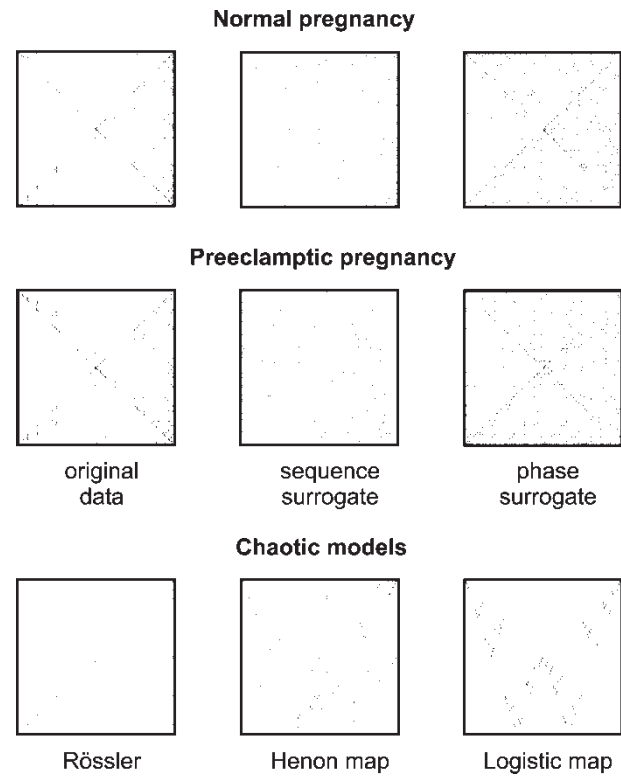
FIGURE 5 IFS clumpiness test applied to the original and surrogate HR data as well as to chaotic models. The first two rows represent the results obtained from the original HR data (left) and the corresponding sequence (middle) and phase (right) surrogate data. The first row corresponds to normal pregnancies while the second one to pre-eclamptic patient. The third row shows the behavior of distinct chaotic models: Rössler attractor (left), Hénon map (middle) and Logistic map (right).
