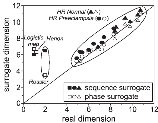
FIGURE 4 Plot of the dependence between the estimated correlation dimension of original data (real dimension) compared to that of surrogate data (surrogate dimension) corresponding to HR recording from healthy and pre-eclamptic pregnant women, Rössler, Hénon and Logistic attractors (chaotic models).
