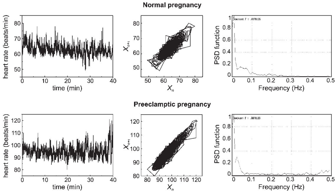
FIGURE 1 The heart rate (HR) sequences (left), reconstructed two dimensional phase-space plots (middle) and power spectra (right) of a healthy and a pre-eclamptic patient.
