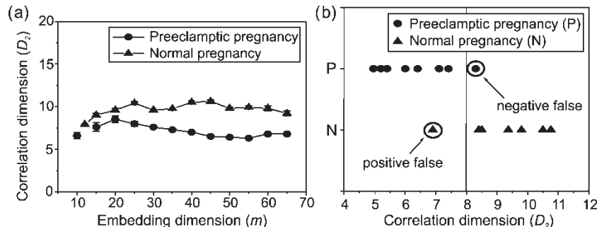
FIGURE 2 (a) Plot of the estimated correlation dimension D_2 from the original HR data versus the embedding dimension, m . (b) Estimated values of the D_2 correlation dimension obtained from the original HR recordings.
