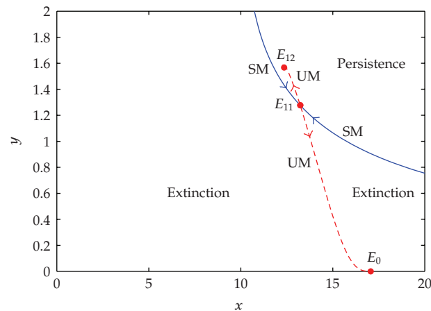
Figure 2: Illustrations of the Allee effect for (1.5). Here, \lambda = 17.06 , d = 1.0 , a = 3.0 , ID_{50} = 2 . E_0 = (17.06, 0) is stable, E_{11} = (13.2311, 1.2763) is a saddle point, E_{12} = (12.3589, 1.567) is stable. Note that SM is the stable manifolds of E_{11} (solid line), UM is the unstable manifolds of E_{11} (dash line), and the phase portrait of (1.6) is divided into two domains of extinction and persistence of the virus by SM.
