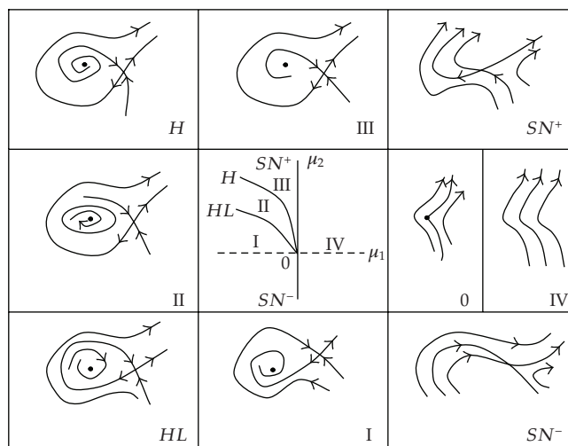
Figure 1: The bifurcation set and the corresponding phase portraits of system (3.26) at origin.
