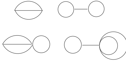
FIG. 1: Symmetry factor for the graphs are 12, 8, 12, 16 respectively
